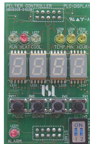
Display board
